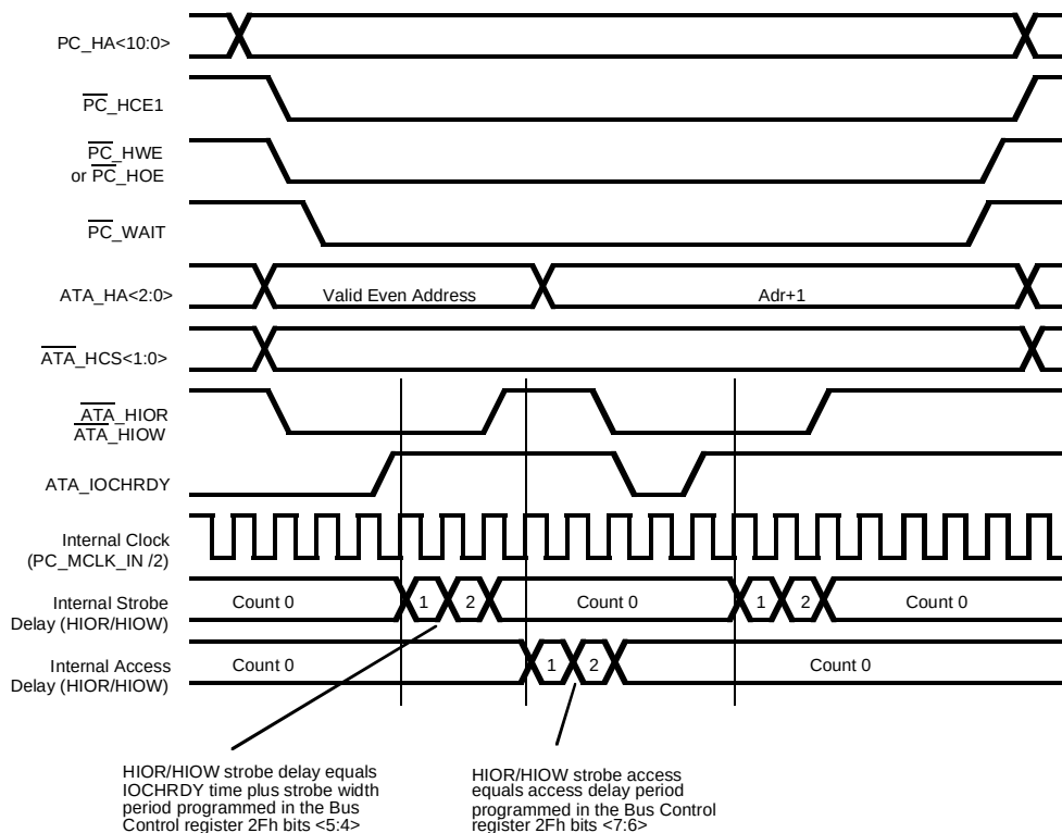
Figure 10. Word-to-Byte Timing
