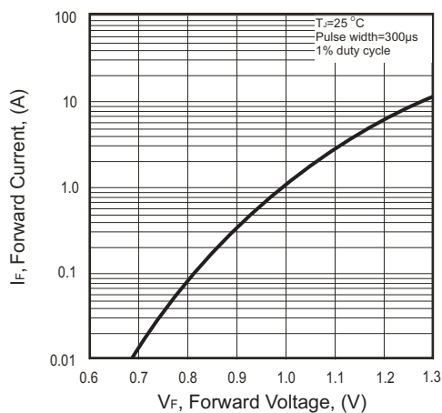
Fig.2 - Forward Characteristics
