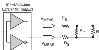
Figure 1-8. Output Delay Timing Reporting Setup modeled by Quartus II Software for Differential Outputs with Three External Resistor
