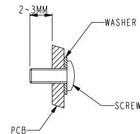
DETAIL 2 RECOMMENDED SCREW LENGTH
