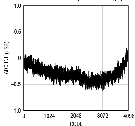
ADC INL vs Code (ADIN Voltage)
