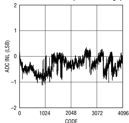
ADC INL vs Code (SENSE Voltage)
