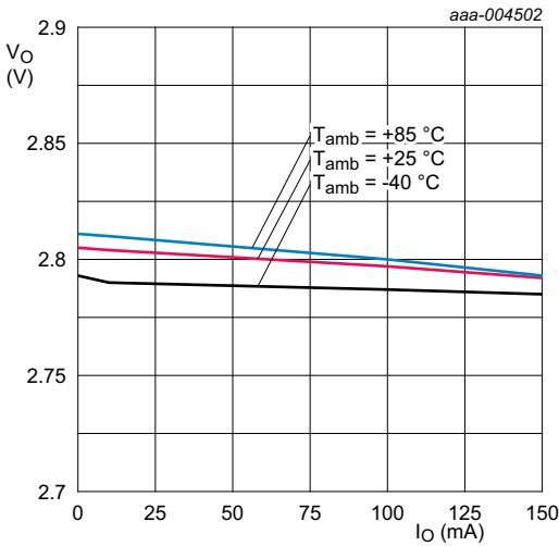
Fig 7. LD6815TD/28x: Output voltage as a function of output current
