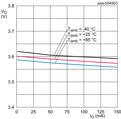
Fig 6. LD6815TD/12x: Output voltage as a function of output current
