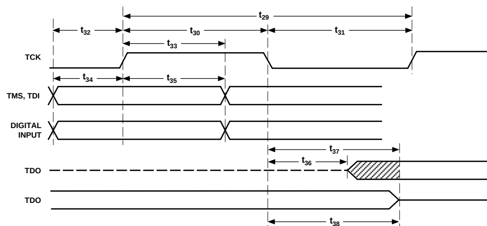
Figure 2. JTAG Timing
