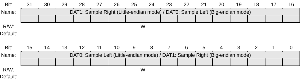
Figure 24-21 ACAUDODAT/ACSURRDAT Register
