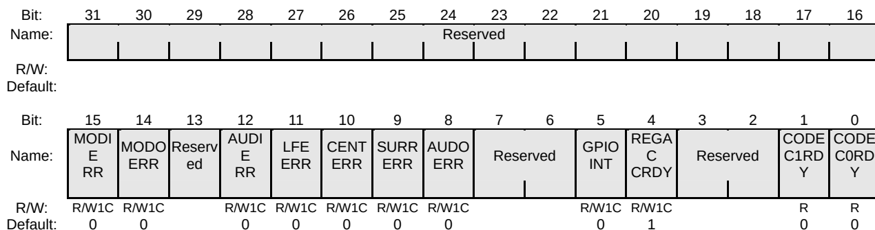
Figure 24-12 ACINTSTS Register
