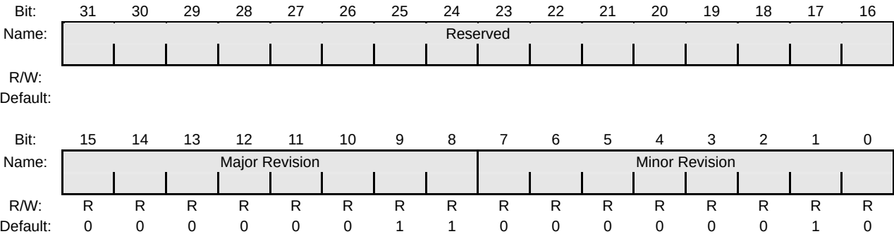
Figure 24-25 ACREVID Register
