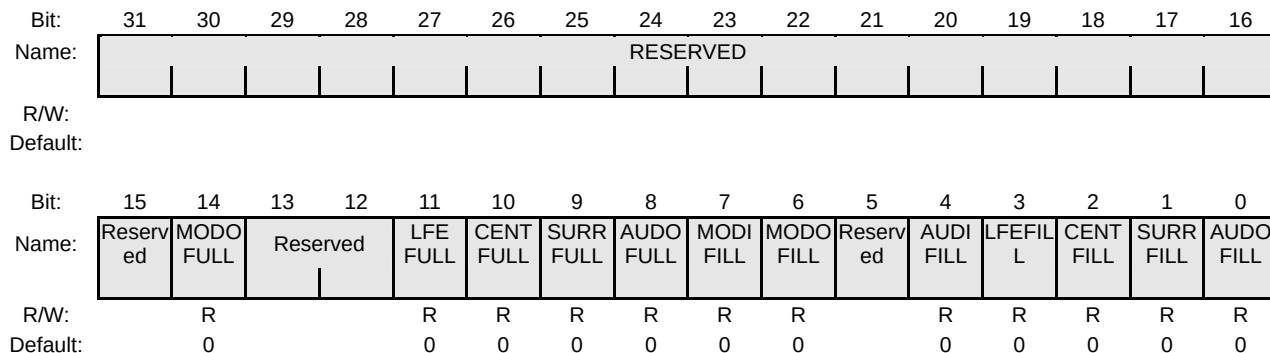
Figure 24-18 ACFIFOSTS Register
