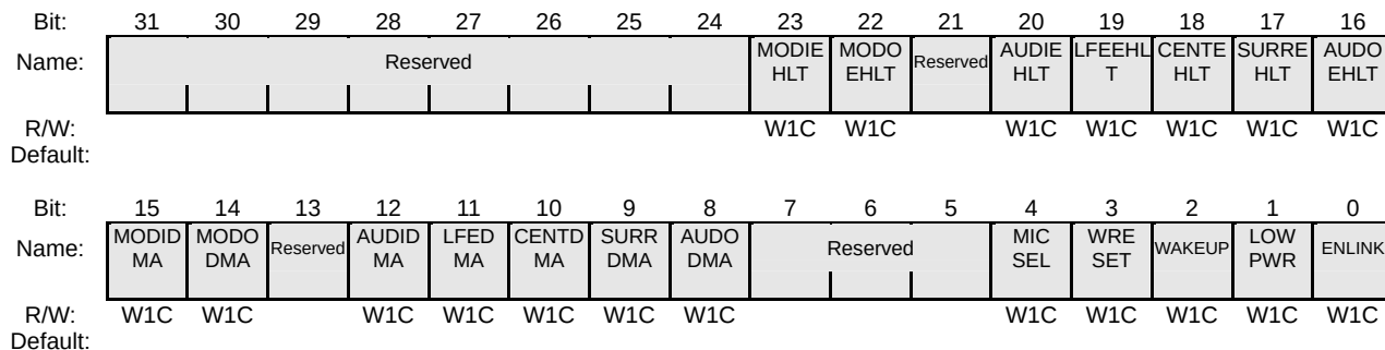
Figure 24-10 ACCTLDIS Register
