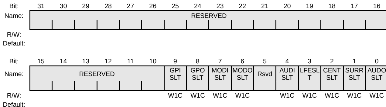
Figure 24-17 ACSLTDIS Register
