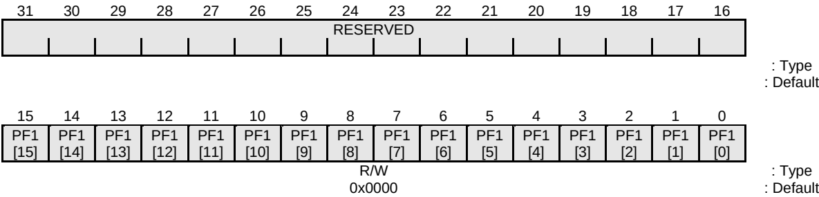
Figure 8-17 Interrupt Request Flag Register 1
