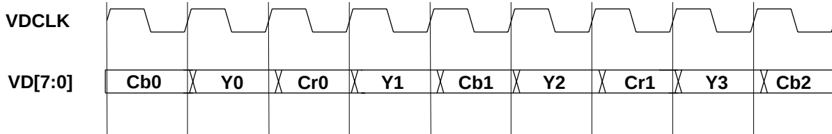
Figure 12-2 ITU.BT656 (CCIR656) Digital Video Timing
