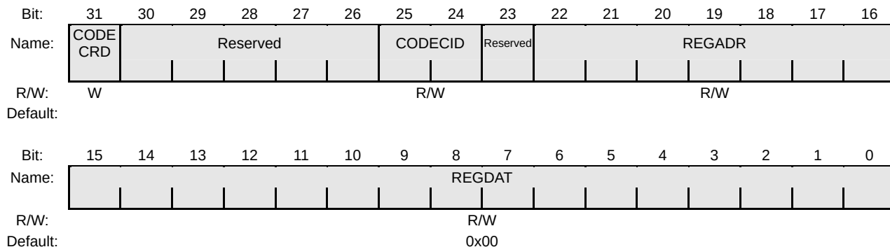
Figure 24-11 ACREGACC
