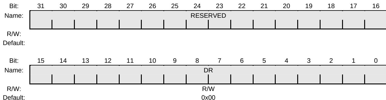
Figure 20-9 SPI Data Register (SPDR)
