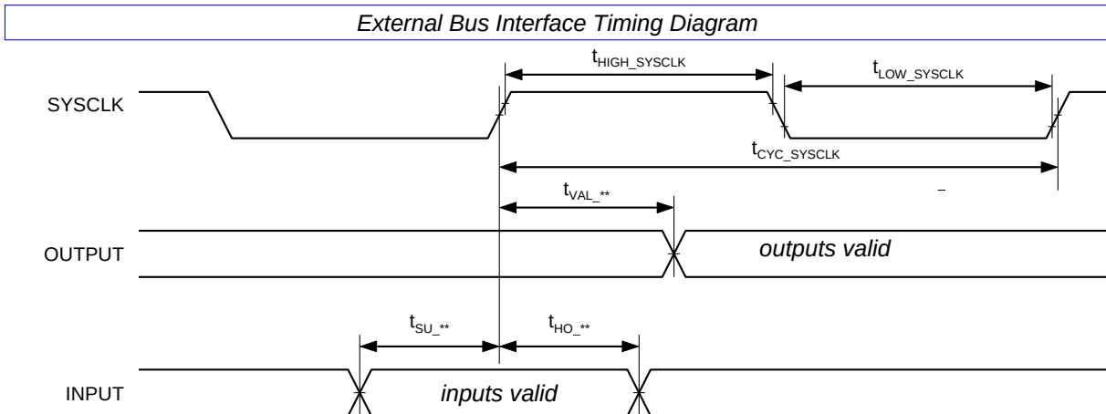
Figure 28-10 External Bus Interface Timing Diagram
