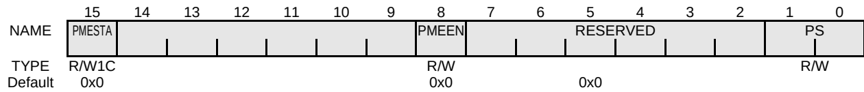
Figure 16-80 PMCSR Register
