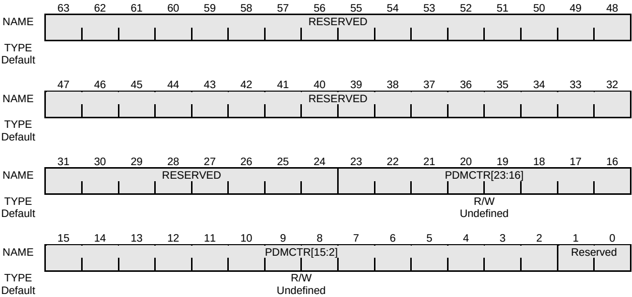
Figure 16-71 Count Register
