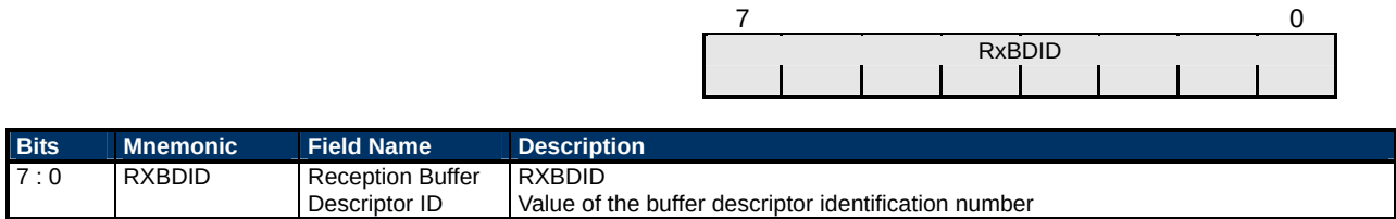
Figure 18-9 BDStat Field
