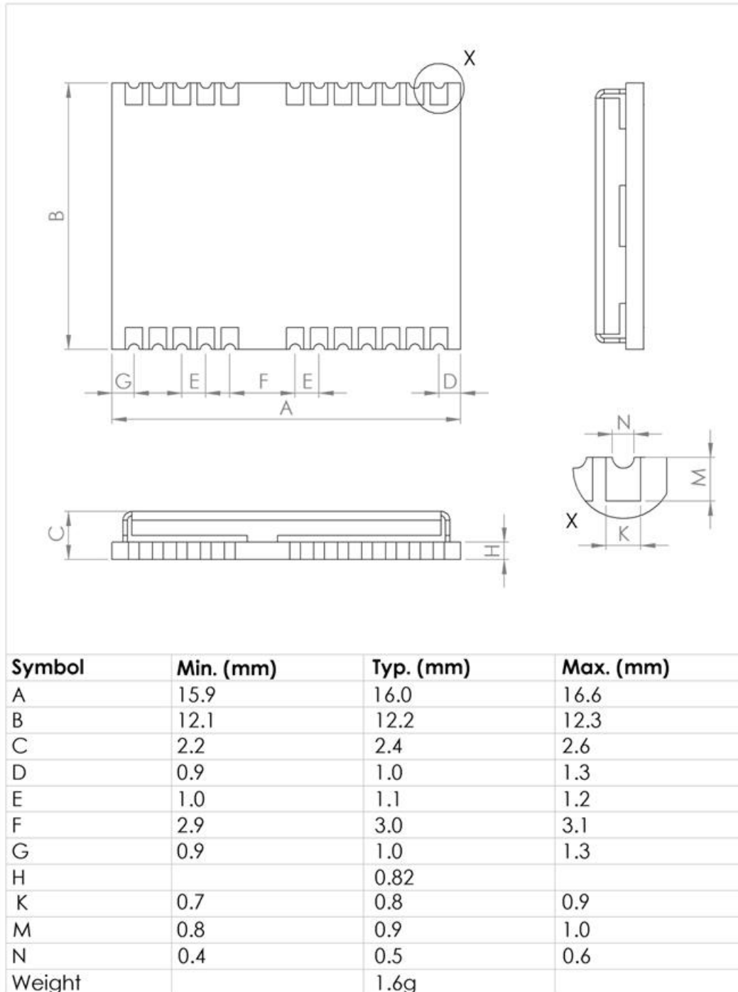
Figure 7: Dimensions
