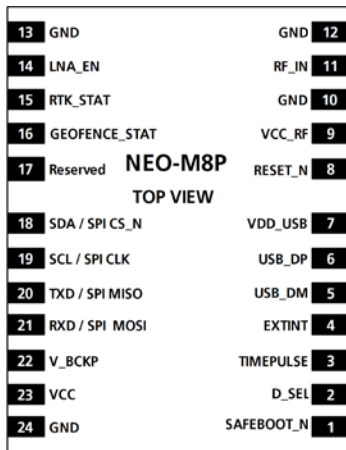
Figure 5: Pin Assignment
