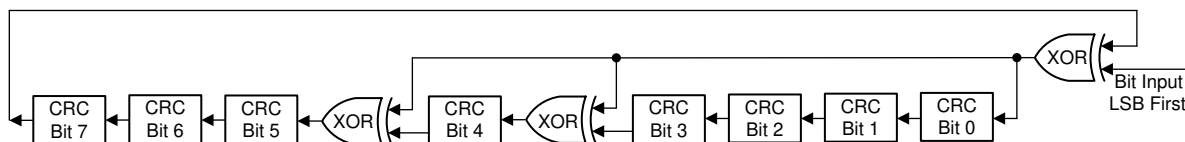
Figure 7-7. CRC Algorithm Diagram
