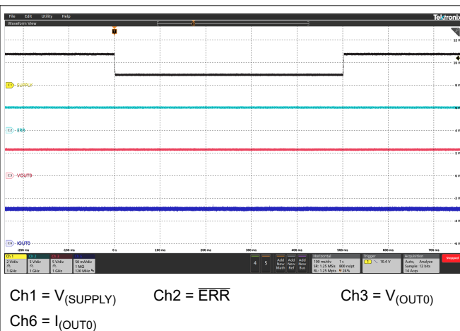
Figure 6-14. Transient Undervoltage
