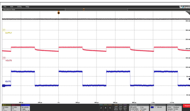
Figure 6-10. LDO Output Load Regulation
