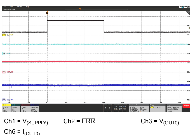
Figure 6-16. Jump Start
