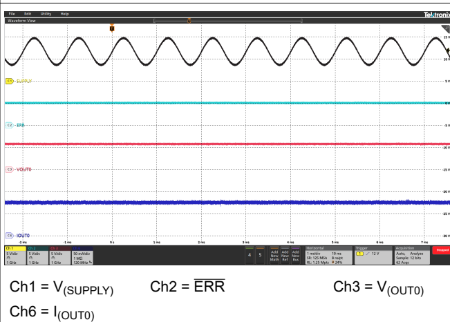
Figure 6-18. Superimposed Alternating Voltage 1 kHz
