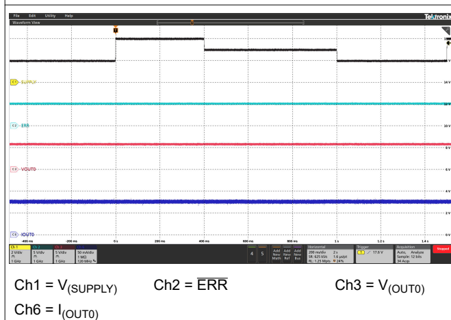
Figure 6-15. Transient Overvoltage
