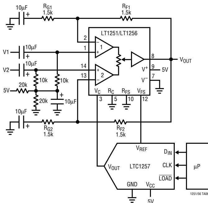
Single Supply Noninverting AC Amplifier with Digital Gain Control
