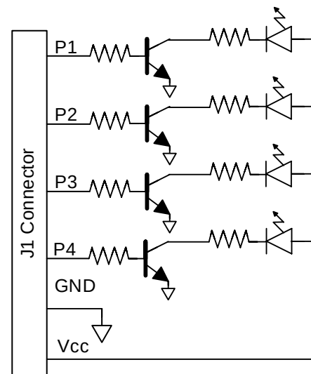
LED Module Circuit Diagram
