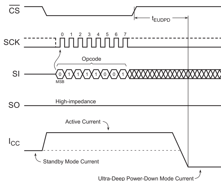
Figure 9-3. Ultra-Deep Power-Down
