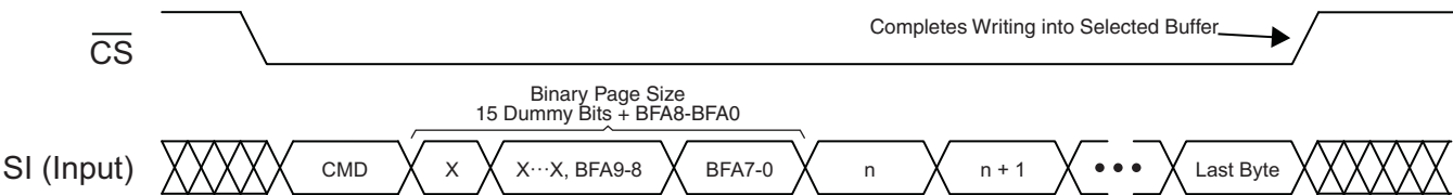
Figure 22-2. Buffer Write
