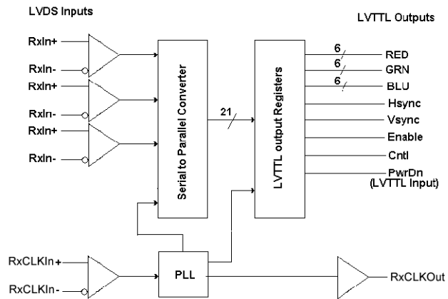
Receiver Functional Diagram for FIN3366 and FIN3364
