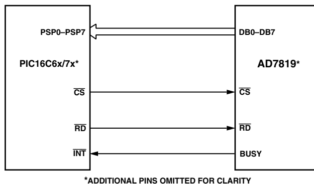
Figure 17. Interfacing to the PIC16C6x/7x
