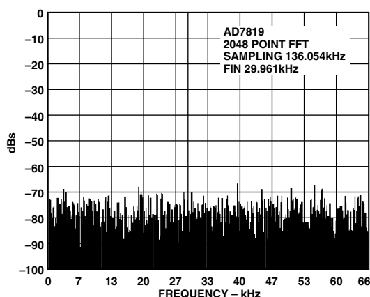
Figure 11. SNR
