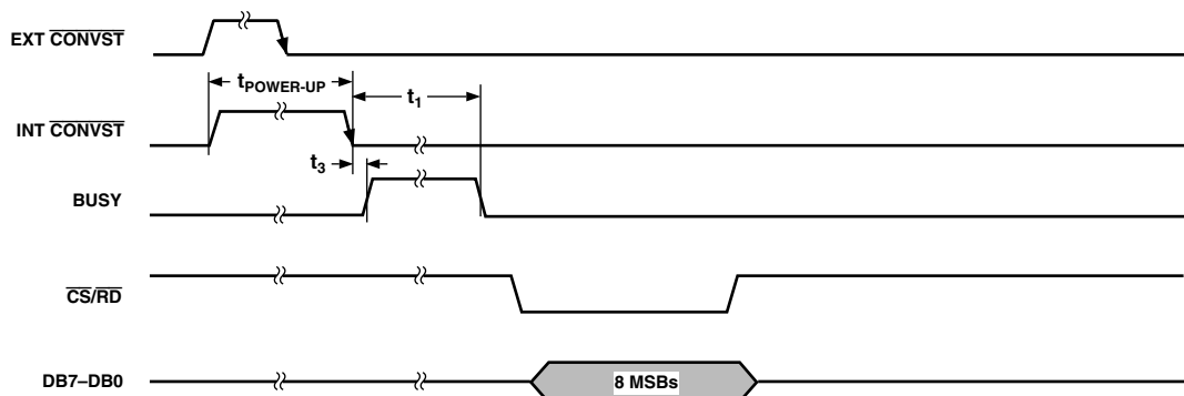
Figure 14. Mode 2 Operation
