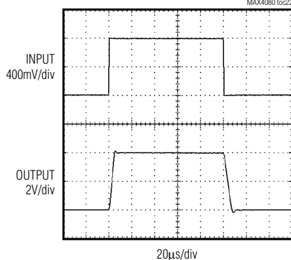
MAX4080F LARGE-SIGNAL TRANSIENT RESPONSE
