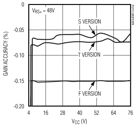
GAIN ACCURACY vs. V_{CC}
