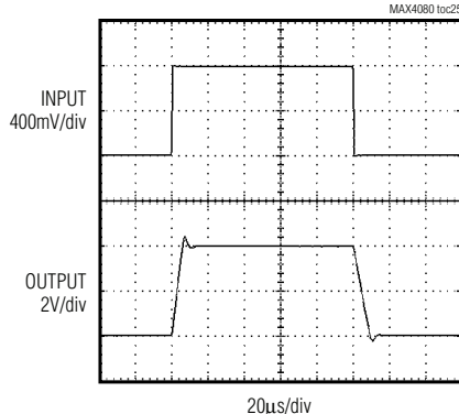
MAX4081F LARGE-SIGNAL TRANSIENT RESPONSE
