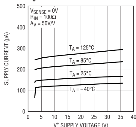
Supply Current vs Supply Voltage, V_S^+ = 0V
