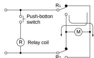
3) R1, R2 : Contacts for R : Double pole relay
