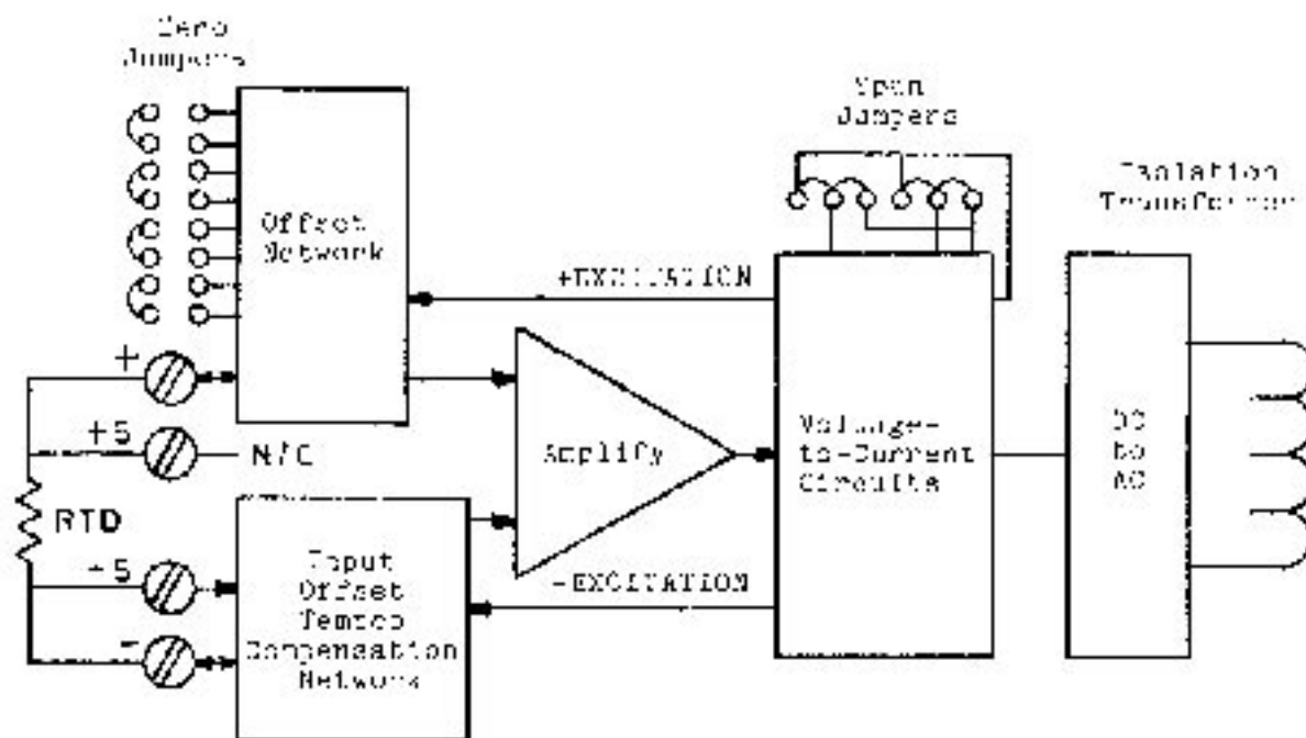
Figure 6-1 502A Preamplifier Block Diagram
