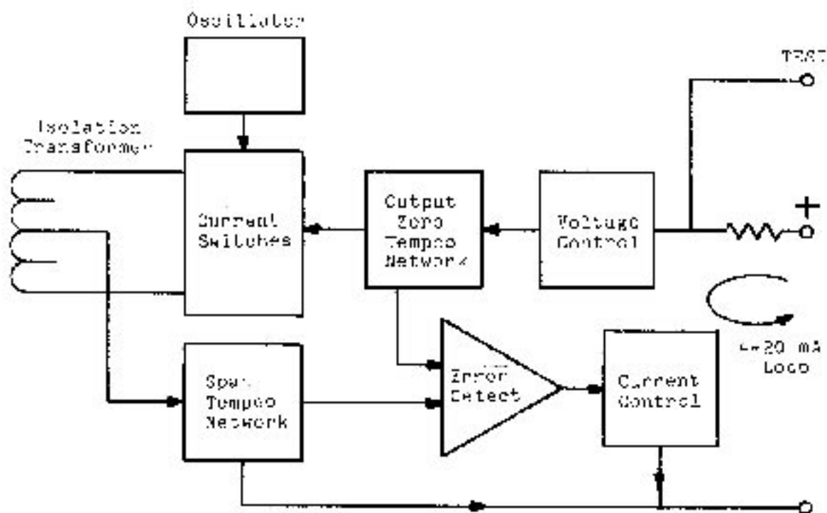
Figure 6-2 502A Postamplifier Block Diagram
