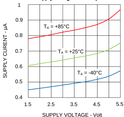
Supply Current vs Supply Voltage and Temperature
