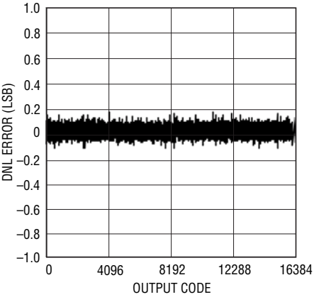
LTC2173-14: Differential Nonlinearity (DNL)
