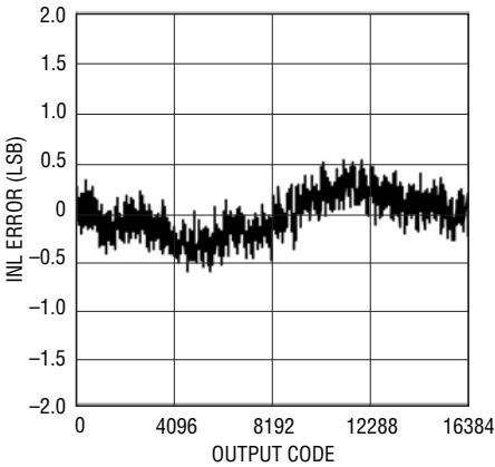
LTC2173-14: Integral Nonlinearity (INL)
