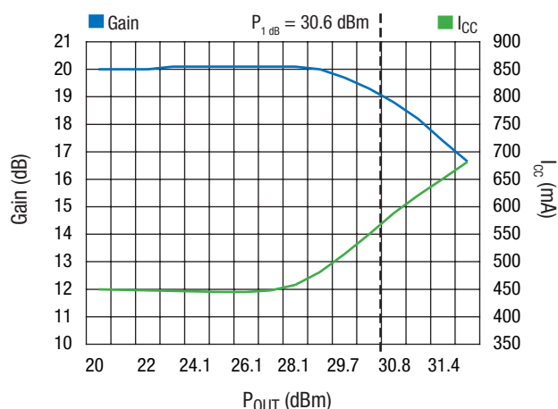
SKY65113 Gain, I_{CC} vs. P_{OUT} V_{CC} = 5.3\text{ V} , V_{REF} = 5\text{ V} , I_{CCQ} = 450\text{ mA} , F = 940\text{ MHz}
