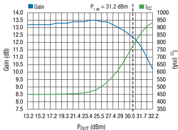
SKY65113 Gain, I_{CC} vs. P_{OUT} V_{CC} = 5\text{ V} , V_{REF} = 5\text{ V} , I_{CCQ} = 450\text{ mA} , F = 1960\text{ MHz}
