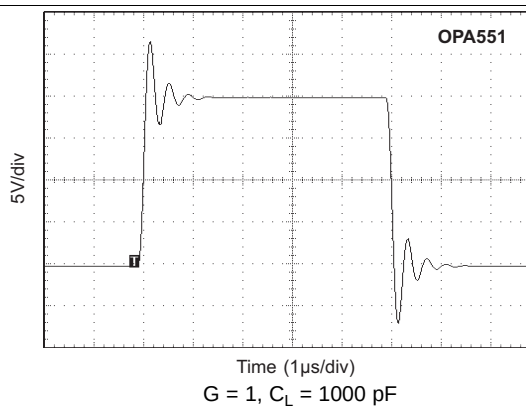
Figure 24. Small-Signal Step Response OPA551
