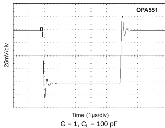
Figure 22. Small-Signal Step Response OPA551
