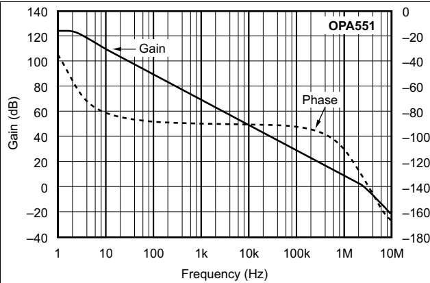
Figure 1. Open-Loop Gain and Phase vs Frequency (OPA551)
