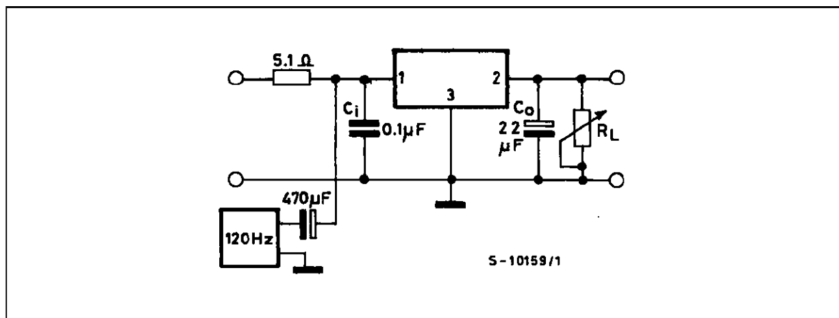
Figure 3 : Ripple Rejection.
