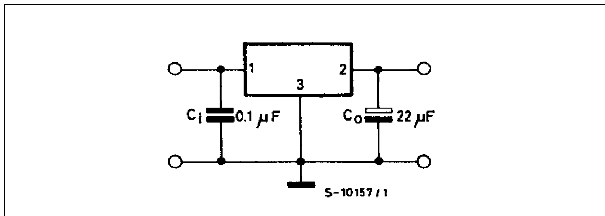
Figure 1 : DC Parameters.
