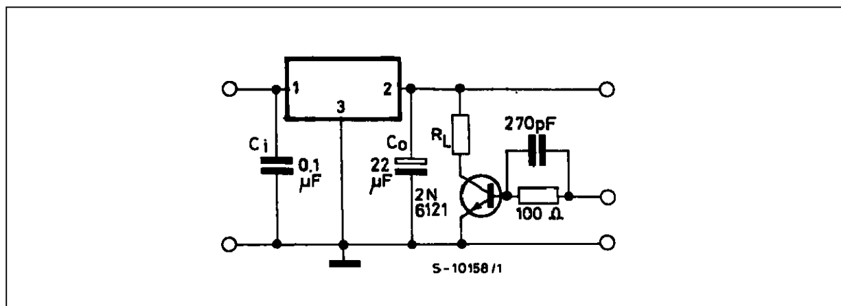
Figure 2 : Load Regulation.
