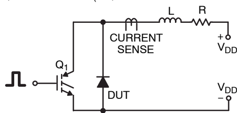
Figure 15. Avalanche Energy Test Circuit
