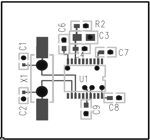
FIGURE 4B. ICS843002-01 PC BOARD LAYOUT EXAMPLE
