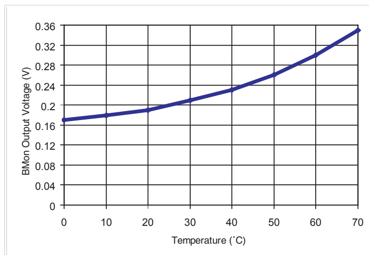
Figure 7 Typical Variations of Bias Monitor Voltage over Temperature
