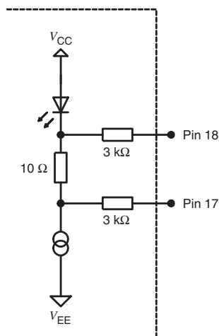
Figure 6 Bias Monitor – Transceiver Internal
