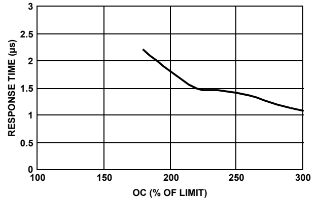
FIGURE 10. RESPONSE TIME vs I_O \cdot R_{SNS}
