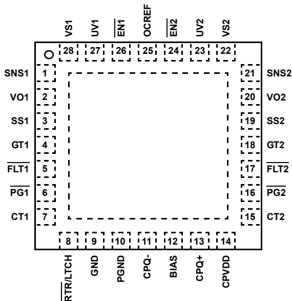
ISL6173 (28 LD QFN) TOP VIEW
