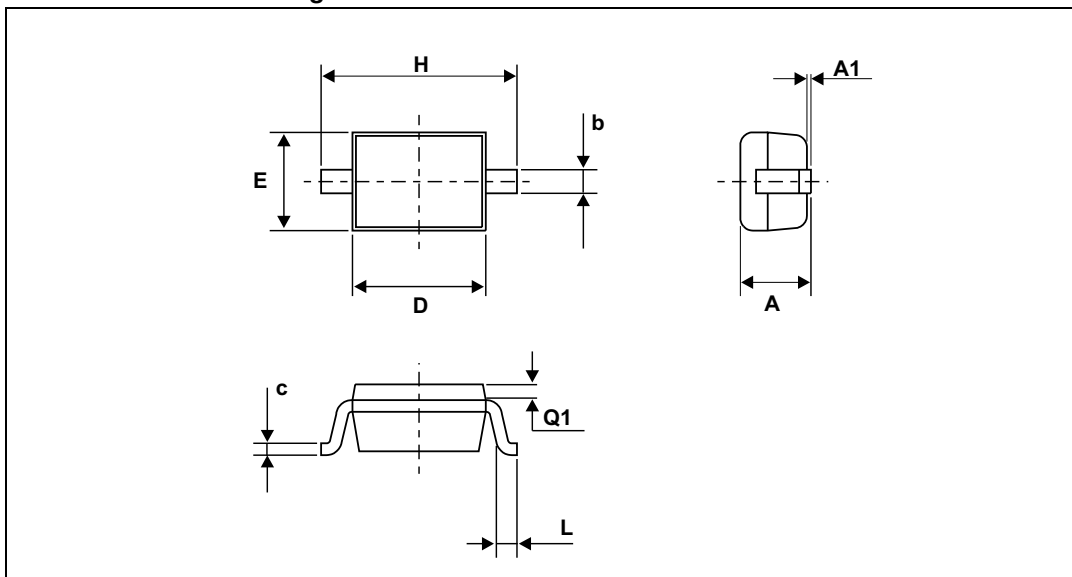
Figure 13. SOD323 dimension definitions
