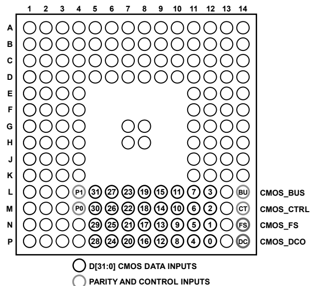
Figure 128. CMOS Data Input Pin Mapping
