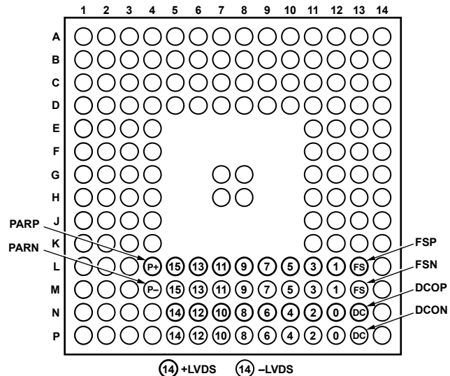
Figure 129. LVDS Data Input Pin Mapping
