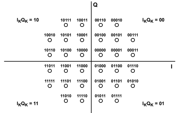
Figure 123. DVB-C 32-QAM Constellation
