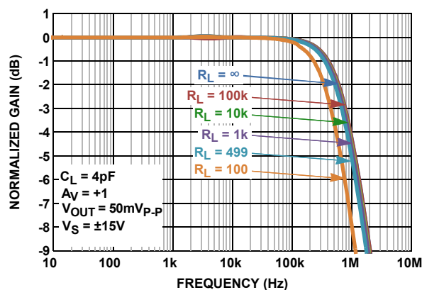
FIGURE 10. UNITY GAIN FREQUENCY RESPONSE vs R_L
