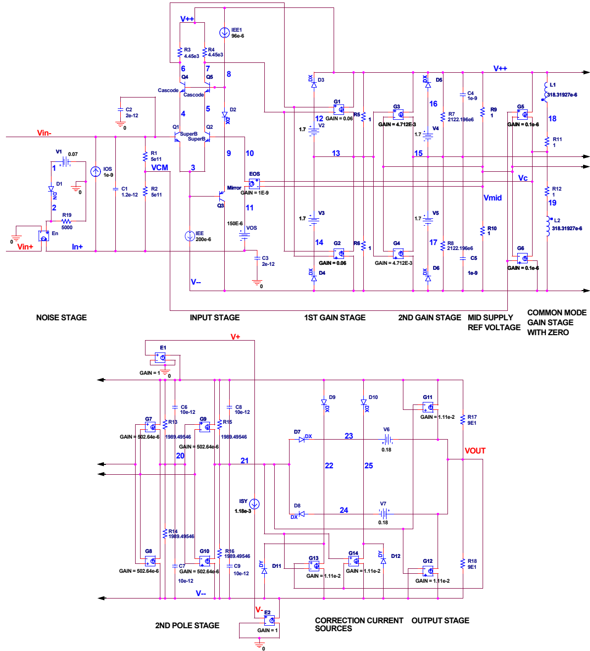
FIGURE 22. SPICE MODEL SCHEMATIC
