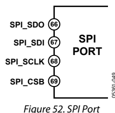
Figure 52. SPI Port
