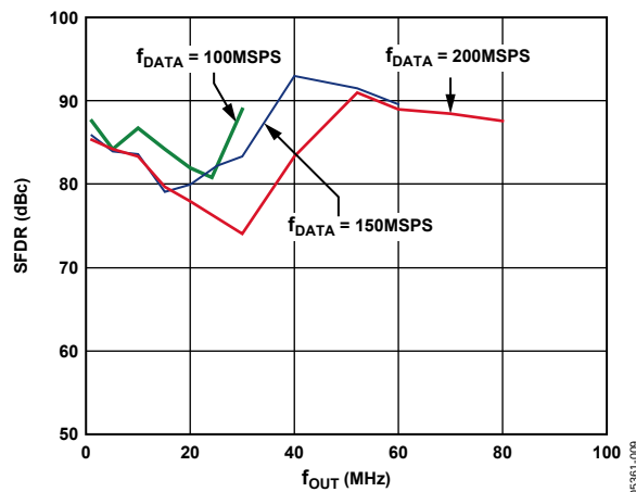
Figure 10. AD9779 In-Band SFDR vs. f_{OUT} , 4x Interpolation
