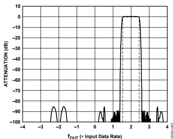
Figure 66. Interpolation/Modulation Combination of 2 f_{DAC}/8 Filter in Shifted Mode
