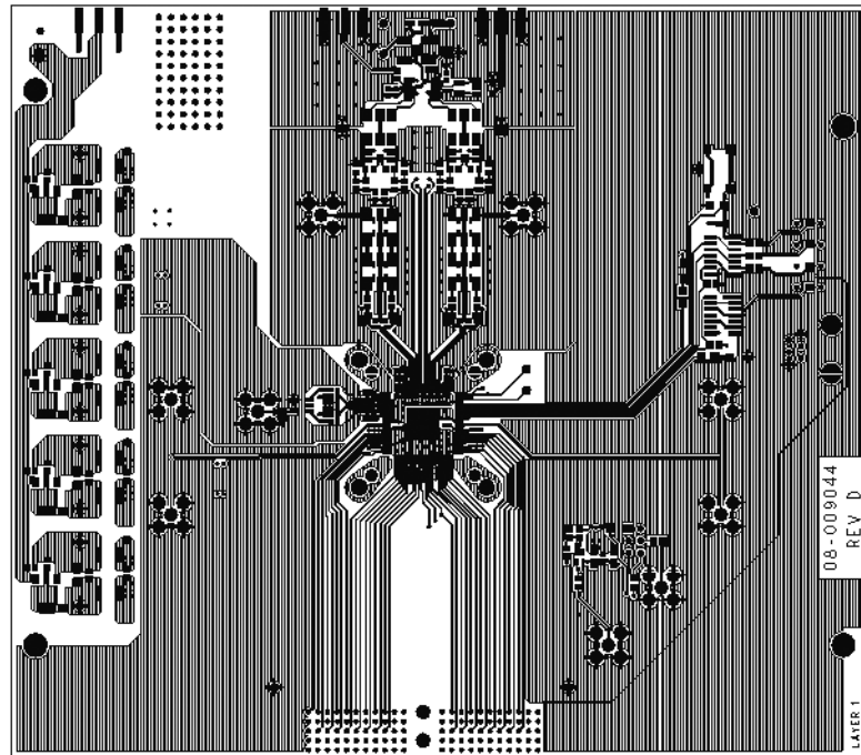
Figure 111. Evaluation Board, Rev. D, Top Layer
