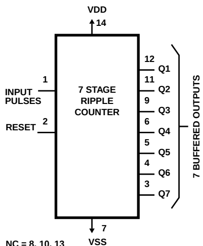
CD4024BMS
