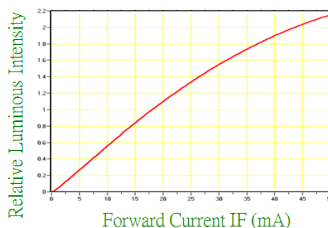
Relative Luminous Intensity-IF (Ta=25°C)
