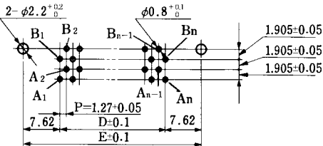
Mating Side
