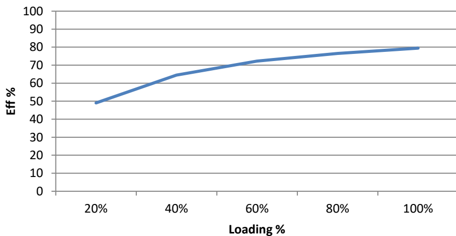
AM1DS-1212SZ Efficiency vs. Loading
