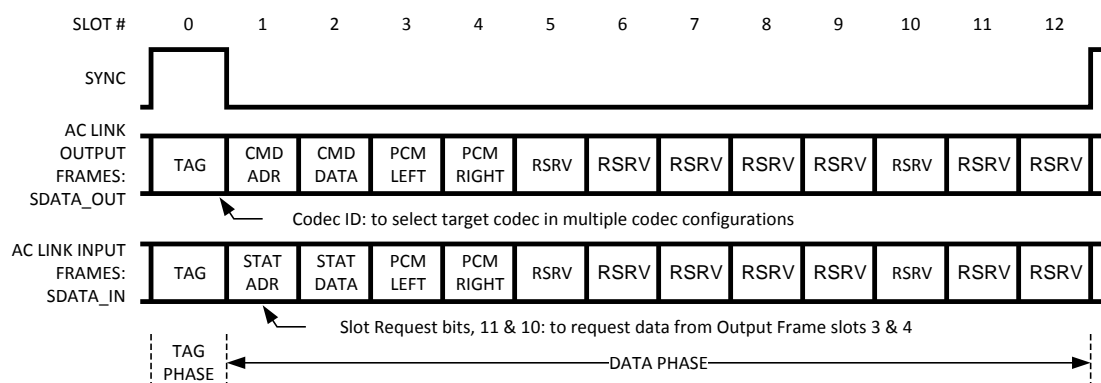
Figure 17. AC Link Bidirectional Audio Frame
