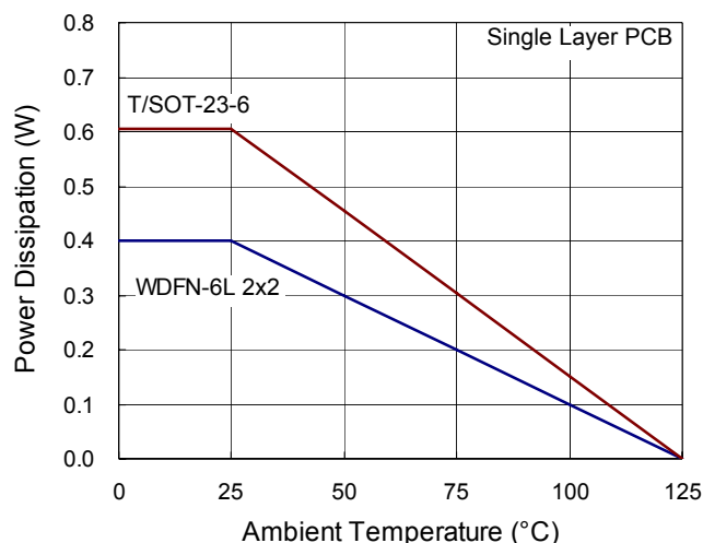
Figure 5. Derating Curves for RT9361 Packages
