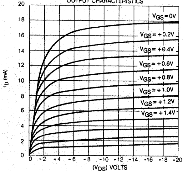
OUTPUT CHARACTERISTICS
