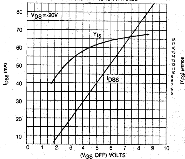
FORWARD TRANSADMITTANCE
