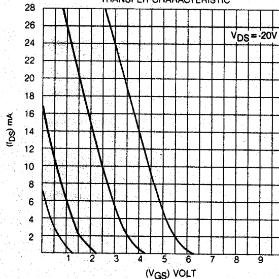
TRANSFER CHARACTERISTIC
