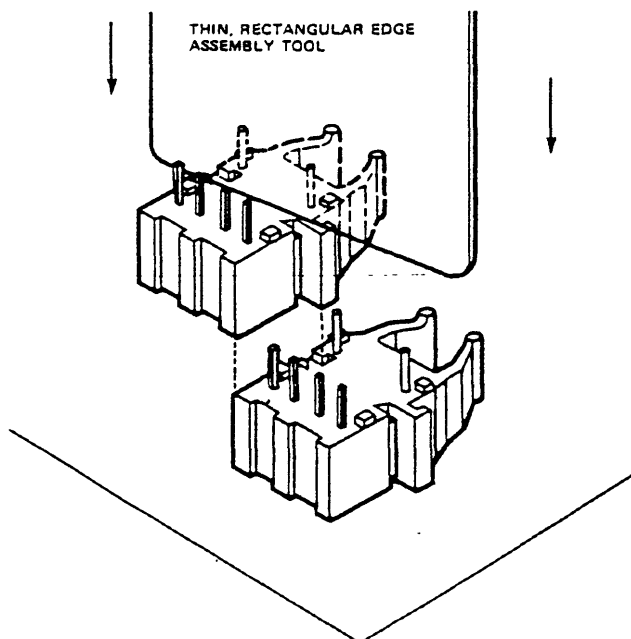
Figure 11. Interlocked (Stacked) Horizontal or Vertical Packages.
