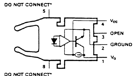
HFBR-25X3 RECEIVER
