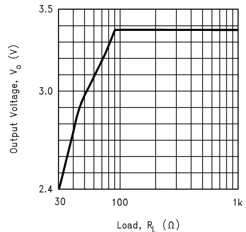
Output Voltage vs. Load
