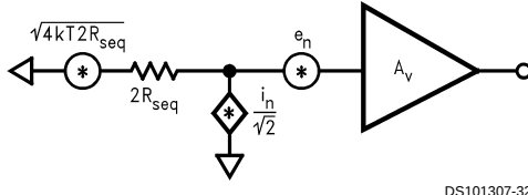
FIGURE 4. Noise Model with R_f \parallel R_g = R_{seq}
