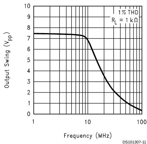
Maximum Output Swing vs. Frequency
