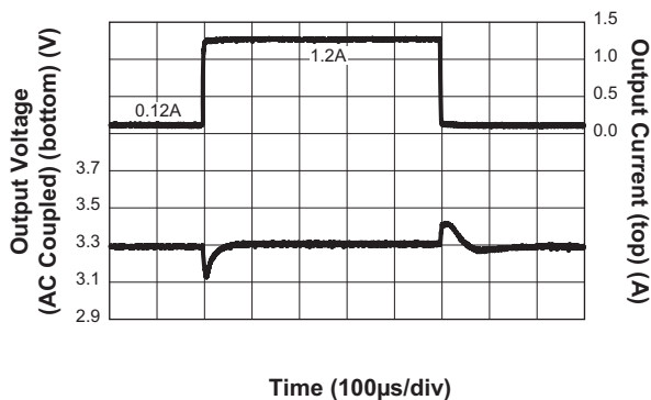
Step-Down Converter Load Transient Response ( I_{OUT} = 0.12A to 1.2A ; V_{IN} = 12V ; V_{OUT} = 3.3V ; C_{OUT} = 2x22\mu F )
