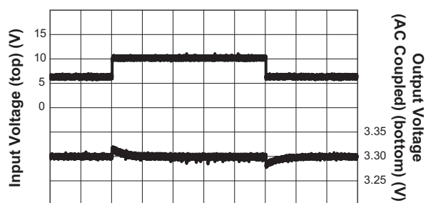
Step-Down Converter Line Transient Response ( V_{IN} = 6V to 10V ; V_{OUT} = 3.3V ; I_{OUT} = 1.2A )
