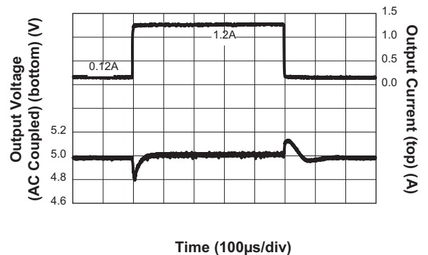
Step-Down Converter Load Transient Response ( I_{OUT} = 0.12A to 1.2A ; V_{IN} = 12V ; V_{OUT} = 5V ; C_{OUT} = 2x22\mu F )
