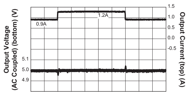
Step-Down Converter Load Transient Response ( I_{OUT} = 0.9A to 1.2A ; V_{IN} = 12V ; V_{OUT} = 5V ; C_{OUT} = 2 \times 22\mu F )
