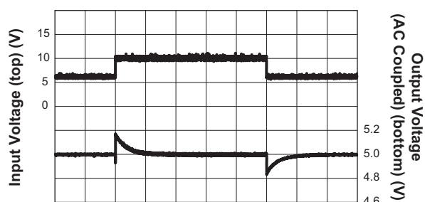
Step-Down Converter Line Transient Response ( V_{IN} = 6V to 10V ; V_{OUT} = 5V ; I_{OUT} = 1.2A )
