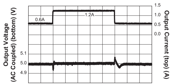
Step-Down Converter Load Transient Response ( I_{OUT} = 0.6A to 1.2A ; V_{IN} = 12V ; V_{OUT} = 5V ; C_{OUT} = 2 \times 22\mu F )
