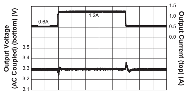
Step-Down Converter Load Transient Response ( I_{OUT} = 0.6A to 1.2A ; V_{IN} = 12V ; V_{OUT} = 3.3V ; C_{OUT} = 2 \times 22\mu F )
