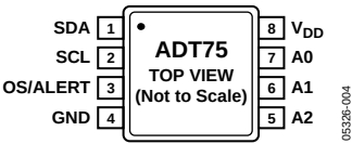
Figure 4. Pin Configuration
