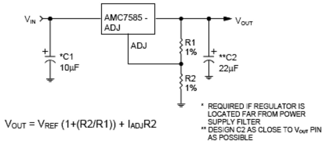
AMC7585-ADJ application schematic
