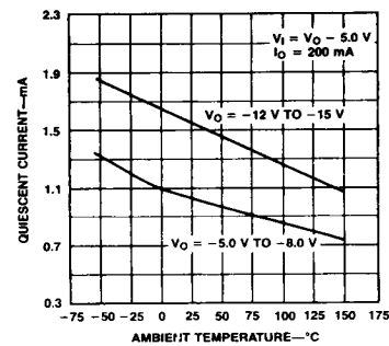
Quiescent Current vs Ambient Temperature
