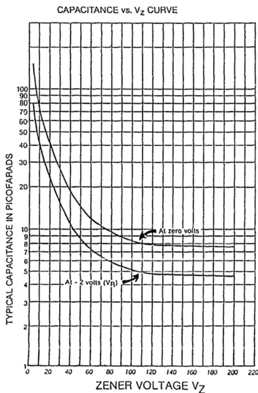
FIGURE 2 CAPACITANCE vs. ZENER VOLTAGE (TYPICAL)
