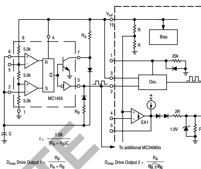
Figure 18. External Duty Cycle Clamp and Multi-Unit Synchronization
