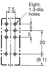
Mounting Holes
