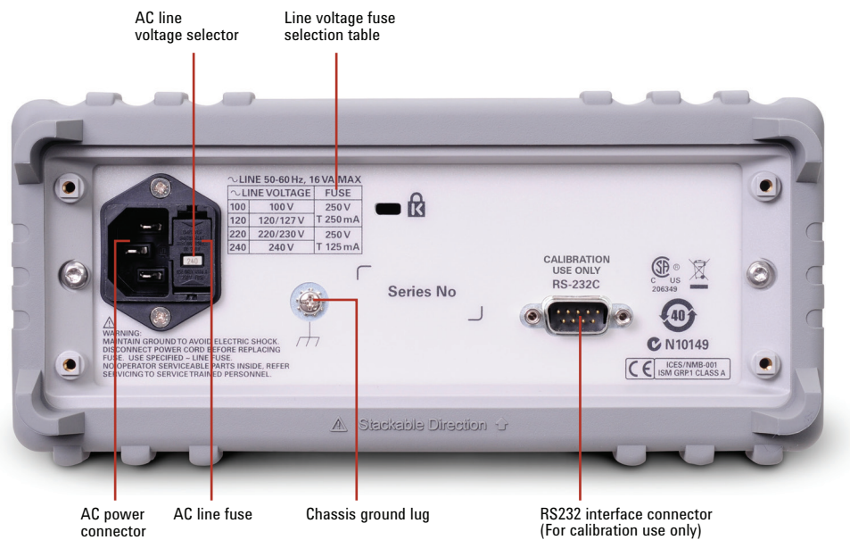
Figure 2 Rear panel of the U3401A/U3402A.
