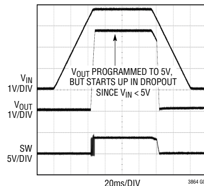
V_{IN} = 0\text{V} TO 3.8V THEN BACK TO 0V I_{LOAD} = 100\text{mA} FIGURE 8 CIRCUIT
